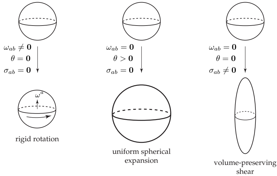
Figure 2.8.2: Rotation, Expansion, Shear
