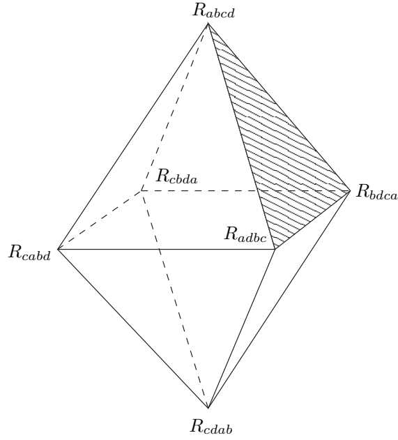
Figure 1.9.1: Symmetries of the Riemann tensor field R_{abcd} .
