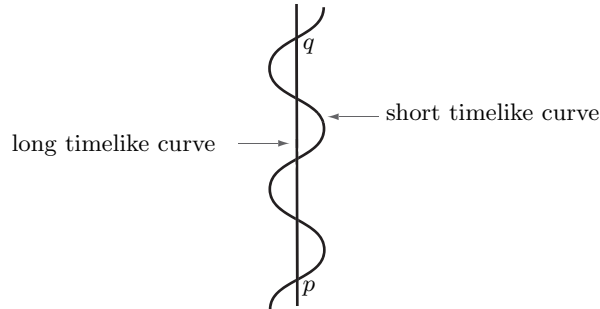
Figure 2.3.1: A long timelike curve from p to q and a very short one that approximates a broken null curve.
