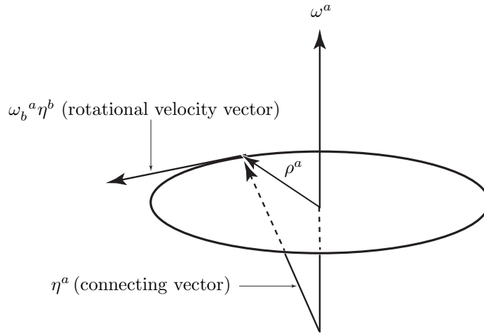
Figure 2.8.1: The angular velocity (or twist) vector \omega^a . It points in the direction of the instantaneous axis of rotation of the fluid. Its magnitude \|\omega^a\| is the instantaneous angular speed of the fluid about that axis. Here \eta^a connects the fluid element O to the “infinitesimally close” fluid element N . The rotational velocity of N relative to O is given by \omega_b{}^a \eta^b . The latter is orthogonal to \eta^a .
