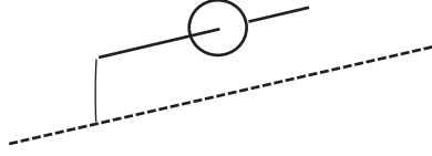
Figure 3.2.6: A gyroscope moving in a “straight line” will not change direction relative to that line.
