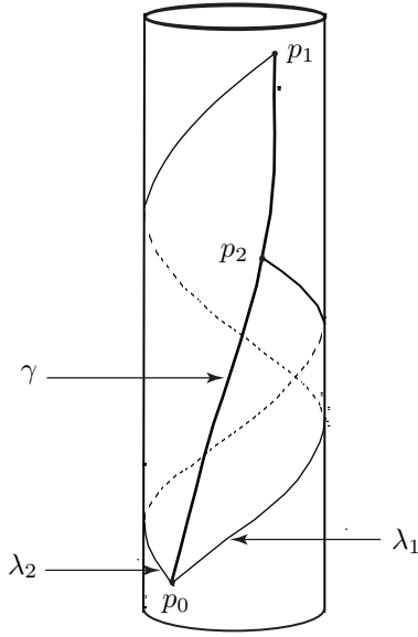
Figure 3.2.5: Sagnac effect.
