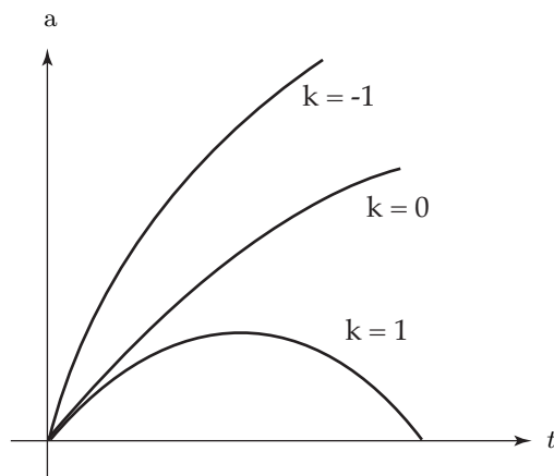
Figure 2.11.1: Rough graphs of the scaling factor a in the three cases.
