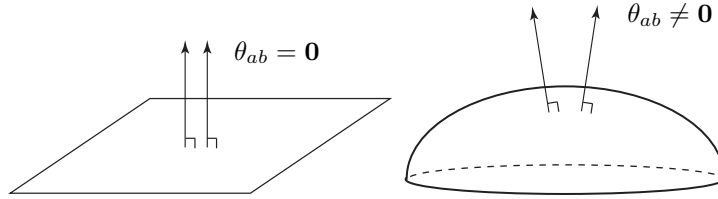
Figure 2.8.3: Expansion and Extrinsic Curvature
