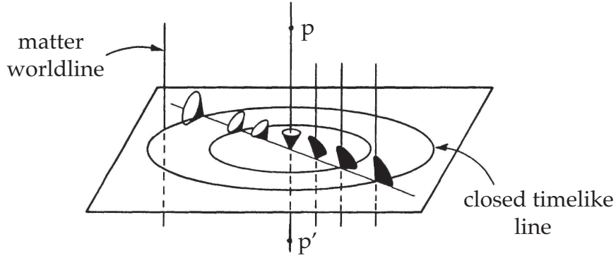
Figure 3.1.1: Gödel spacetime with one dimension (the \tilde{z} dimension) suppressed.
