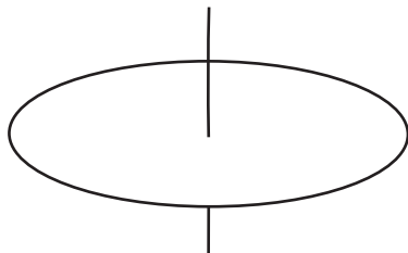
Figure 3.2.1: What does it mean to say that a ring is “not rotating” around a central axis of rotational symmetry?
