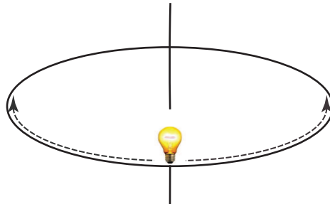
Figure 3.2.4: An experimental test to determine whether the ring is non-rotating according to the ZAM (zero angular momentum) criterion.
