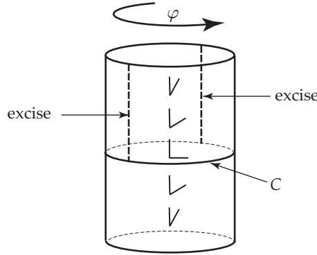
Figure 2.2.2: An example of a spacetime that is future distinguishing but not past distinguishing. Let \varphi be a bijection of the spacetime onto itself that leaves the lower open half below C fixed but reverses the position of the two upper slabs. It is a \ll -isomorphism, but it is discontinuous along C .
