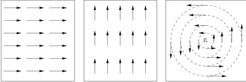
Figure 1.9.2: Killing fields in the Euclidean plane.
