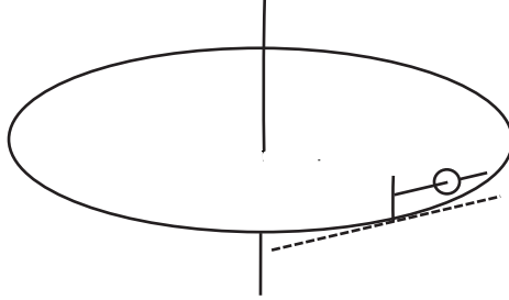
Figure 3.2.3: An experimental test to determine whether the ring is non-rotating according to the CIR (compass of inertia on the ring) criterion.
