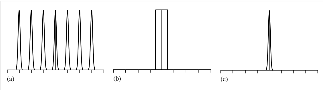
Figure 7.7: Multiplying (a) a series of copies of F(\omega) by (b) the appropriate box function yields (c) the original spectrum.
