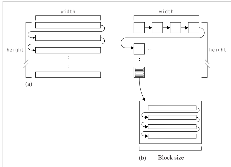
Figure A.2: (a) In C++, the natural layout for a 2D array of size \text{width} \times \text{height} entries, where the (u, v) array element is at the u+v \times \text{width} offset. (b) A blocked array has been split into smaller square blocks, each of which is laid out linearly. Although it is slightly more complex to find the memory location associated with a given (u, v) array position in the blocked scheme, the improvement in cache performance due to more coherent memory access patterns often more than makes up for this in overall faster performance.
