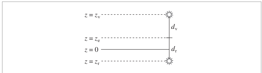
Figure 15.17: Basic Setting for the Dipole Approximation to the Solution to the Diffusion Equation. A light source with positive flux is placed at a position z = z_r inside the medium, below the point where incident illumination arrives, and a second light with an equal amount of negative flux is placed at z = z_v above the medium. These sources are placed so that the flux for the two of them cancels out at a height z_e above the boundary, fulfilling the linearized boundary condition. The fluence rate that results from subtracting the closed-form solution for each of them, Equation (15.25), at the medium's boundary z = 0 is a reasonable approximation of the fluence rate at the boundary due to subsurface scattering.
