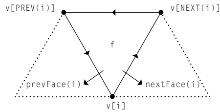
Figure 3.29: Given a vertex v[i] and a face that it is incident to, f , we define the next face as the face adjacent to f across the edge from v[i] to v[\text{NEXT}(i)] . The previous face is defined analogously.
