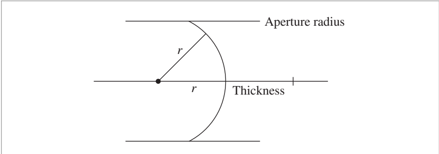
Figure 6.18: A lens interface (solid curved line) intersecting the optical axis at a position z . The interface geometry is described by the interface's aperture radius, which describes its extent above and below the optical axis, and the element's curvature radius r . If the element has a spherical cross section, then its profile is given by a sphere with center a distance r away on the optical axis, where the sphere also passes through z . If r is negative, the element interface is concave as seen from the scene (as is shown here); otherwise it is convex. The thickness of the lens gives the distance to the next interface to the right, or the distance to the film plane for the rearmost interface.
