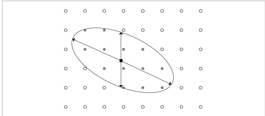
Figure 10.15: The EWA filter applies a Gaussian filter to the texels in an elliptical area around the evaluation point. The extent of the ellipse is such that its edge passes through the positions of the adjacent texture samples as estimated by the texture coordinate partial derivatives.
