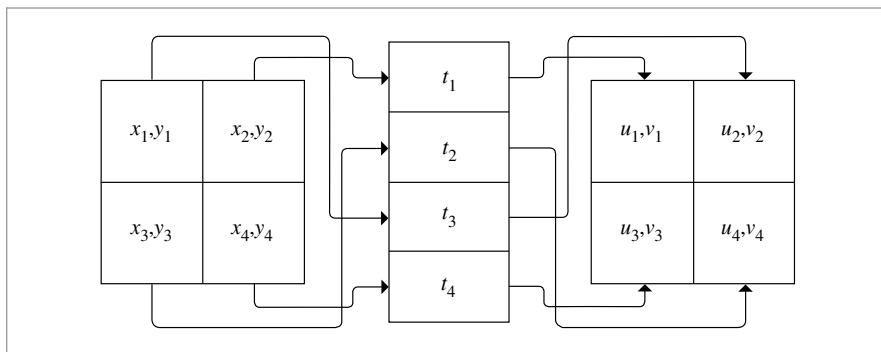
Figure 7.16: We can generate a good sample pattern that reaps the benefits of stratification without requiring that all of the sampling dimensions be stratified simultaneously. Here, we have split (x, y) image position, time t , and (u, v) lens position into independent strata with four regions each. Each is sampled independently, then a time sample and a lens sample are randomly associated with each image sample. We retain the benefits of stratification in each of the individual dimensions without having to exponentially increase the total number of samples.
