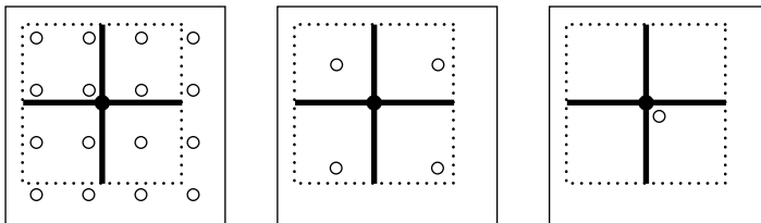
Figure 10.13: Choosing a MIP Map Level for the Triangle Filter. The MIPMap chooses a level such that the filter covers four texels.
