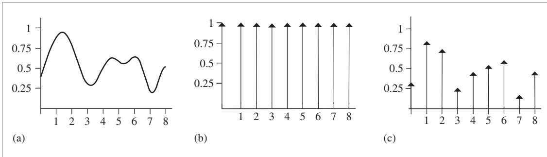
Figure 7.4: Formalizing the Sampling Process. (a) The function f(x) is multiplied by (b) the shah function \text{III}_T(x) , giving (c) an infinite sequence of scaled delta functions that represent its value at each sample point.
