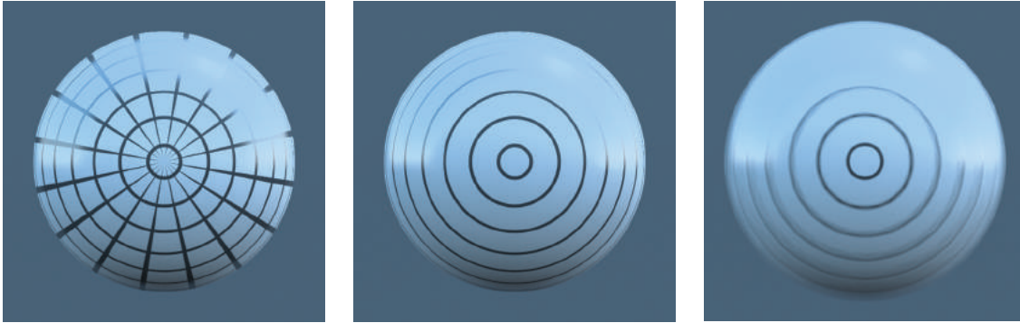
Figure 2.16: (left) Sphere with a grid of lines as a texture, not rotating. (middle) Sphere rotating 90 degrees during the course of the frame, using the technique for interpolating transformations implemented in this section. (right) Sphere rotating 90 degrees using direct interpolation of matrix components to interpolate transformations. In this case, the animated sphere incorrectly grows larger. Furthermore, the lines toward the outside of the sphere, which should remain sharp, incorrectly become blurry.
